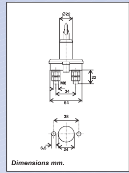
Dimensions mm.
